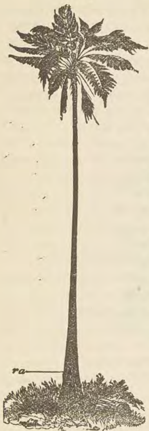
EAST INDIA TREE-FERN.* ( Asophila perrotetiana. )
